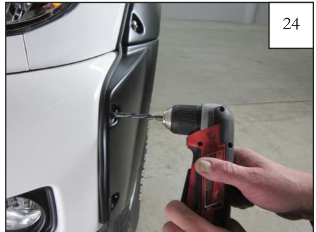
Drill through holes in bumper piece and into sheet metal with a 5/16" drill bit
