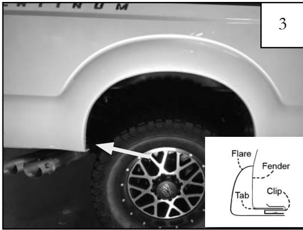
3 Install "S" clip (CL1-0005) over the tab on the rear most hole as shown.
