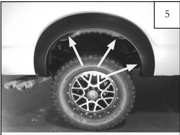
5 Position the flare on the fender and install a 5/8" Phillips Truss Screw (SW1-0058) into each of the three "U" clips installed in the previous step.
