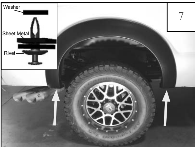
7 On the underside of each end of the flare, install a push retainer (RV1-P009) into the flare hole and then place a washer (WA1-0012) on the backside to hold it in place.
