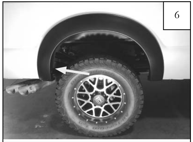
6 Install a 5/16" Phillips Truss Screw (SW1-0050) into the "S" clip over the rear most hole.
